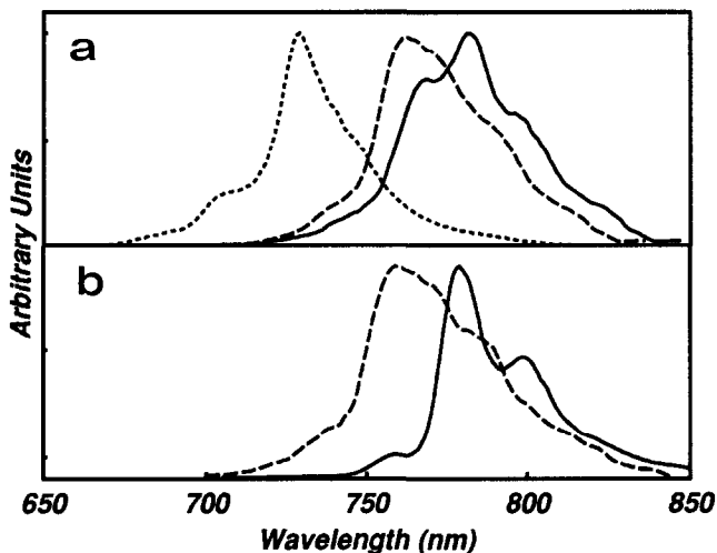
Figure 2. (a) Emission spectral changes during reaction (see text). (dotted line) DMF solution of \text{cis-Ru(bpy)}_3[\text{NC-trans-Cr(cyclam)-CN}]_2^{4+} ; (broken line) upon addition of an excess of \text{Cr(CN)}_6(\text{DMF})_2^{2-} ; (full line) after staying at room temperature for 48 h. (b) Emission spectra of \text{Cr(CN)}_6(\text{DMF})_2^{2-} (broken line) and \text{NC-trans-Cr(cyclam)-CN-Cr(CN)}_5^- (full line)
