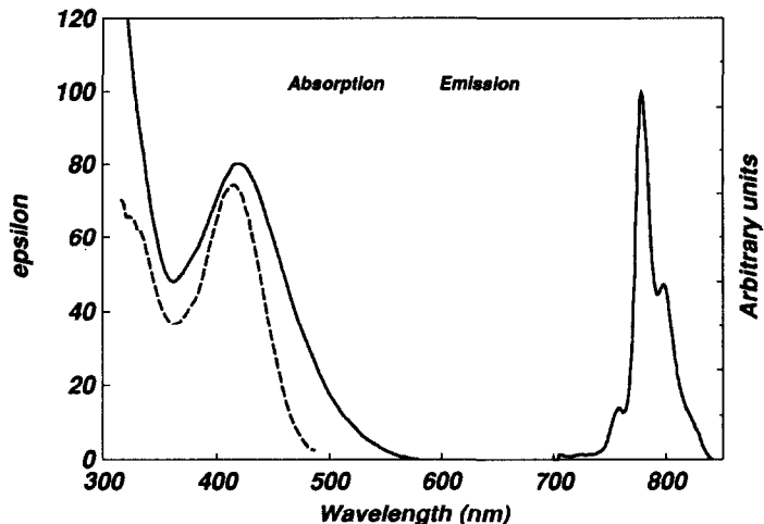
Figure 1. Absorption and emission spectra of \text{NC-trans-Cr(cyclam)-CN-Cr(CN)}_5^- . The broken line represents the excitation spectrum of the emission.
